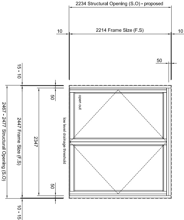
2 No. thus Entrance - unit 2 ref: GFD2, GFD3
