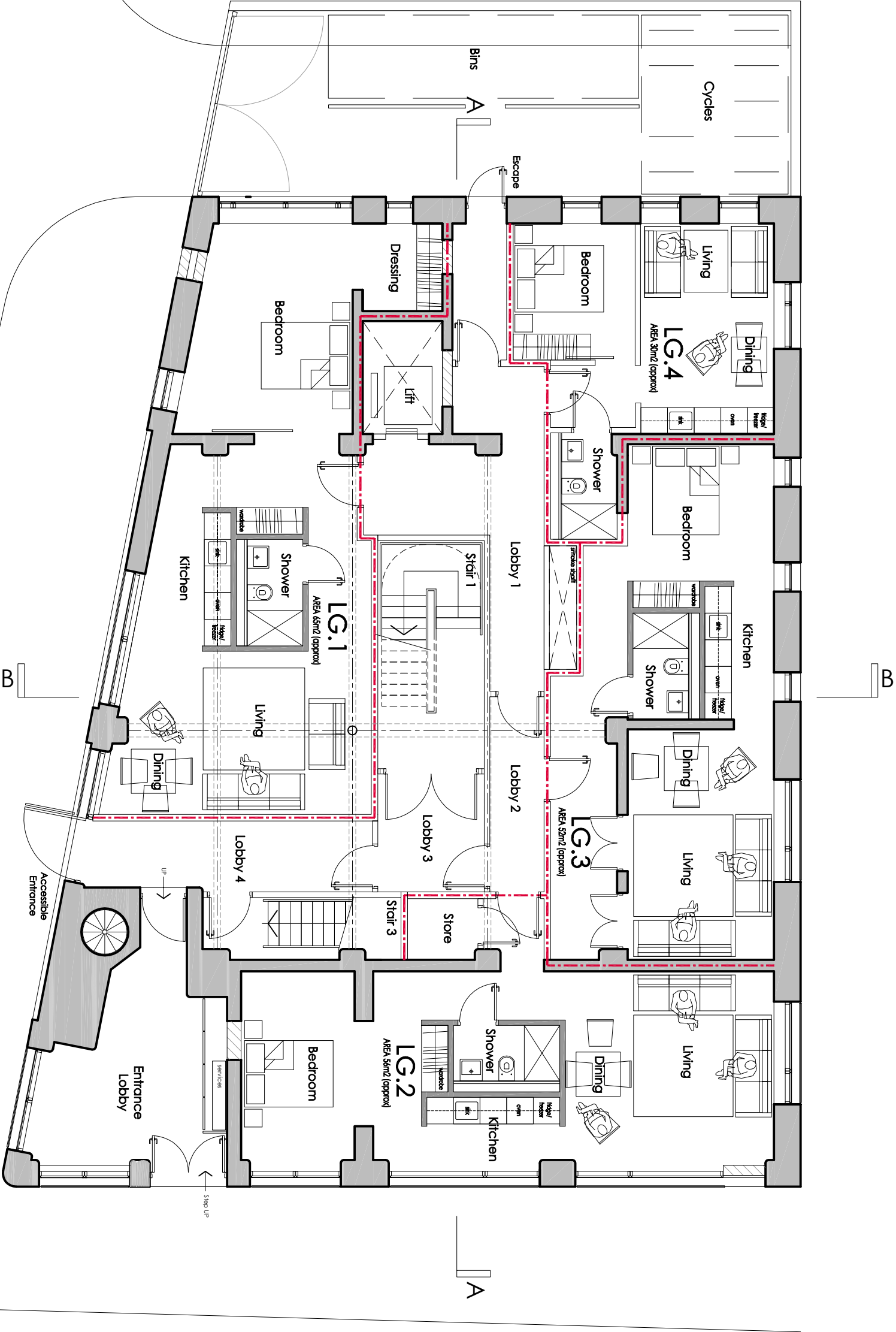
Lower Ground Floor Plan
