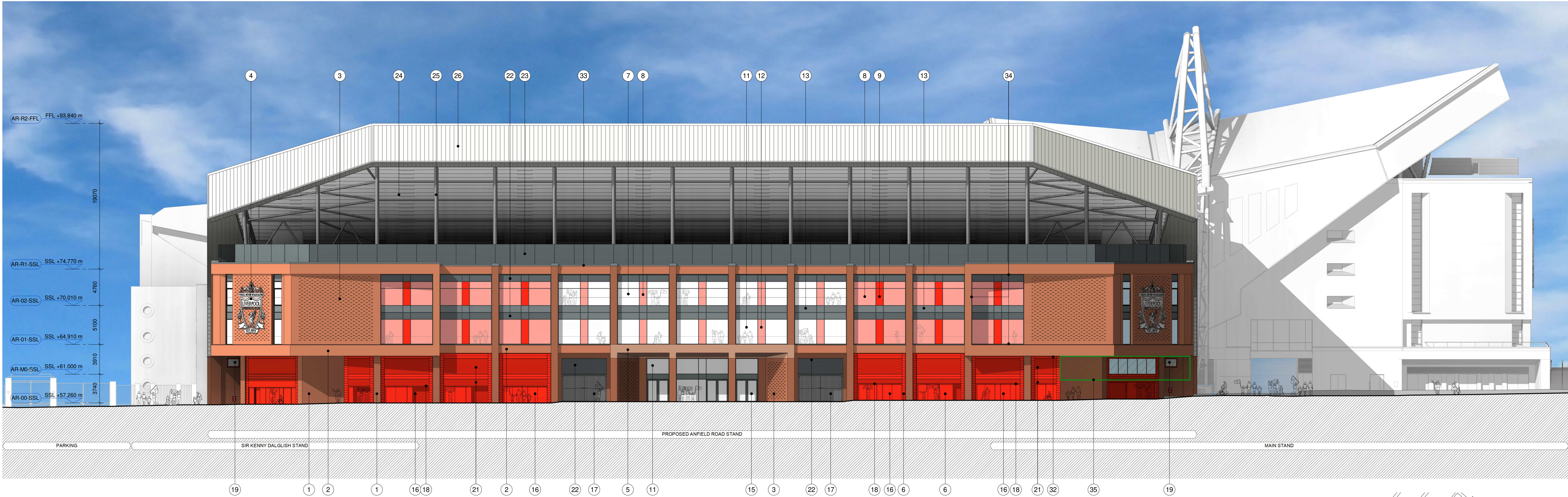
1 PROPOSED NORTH-EAST ELEVATION 1 : 250
