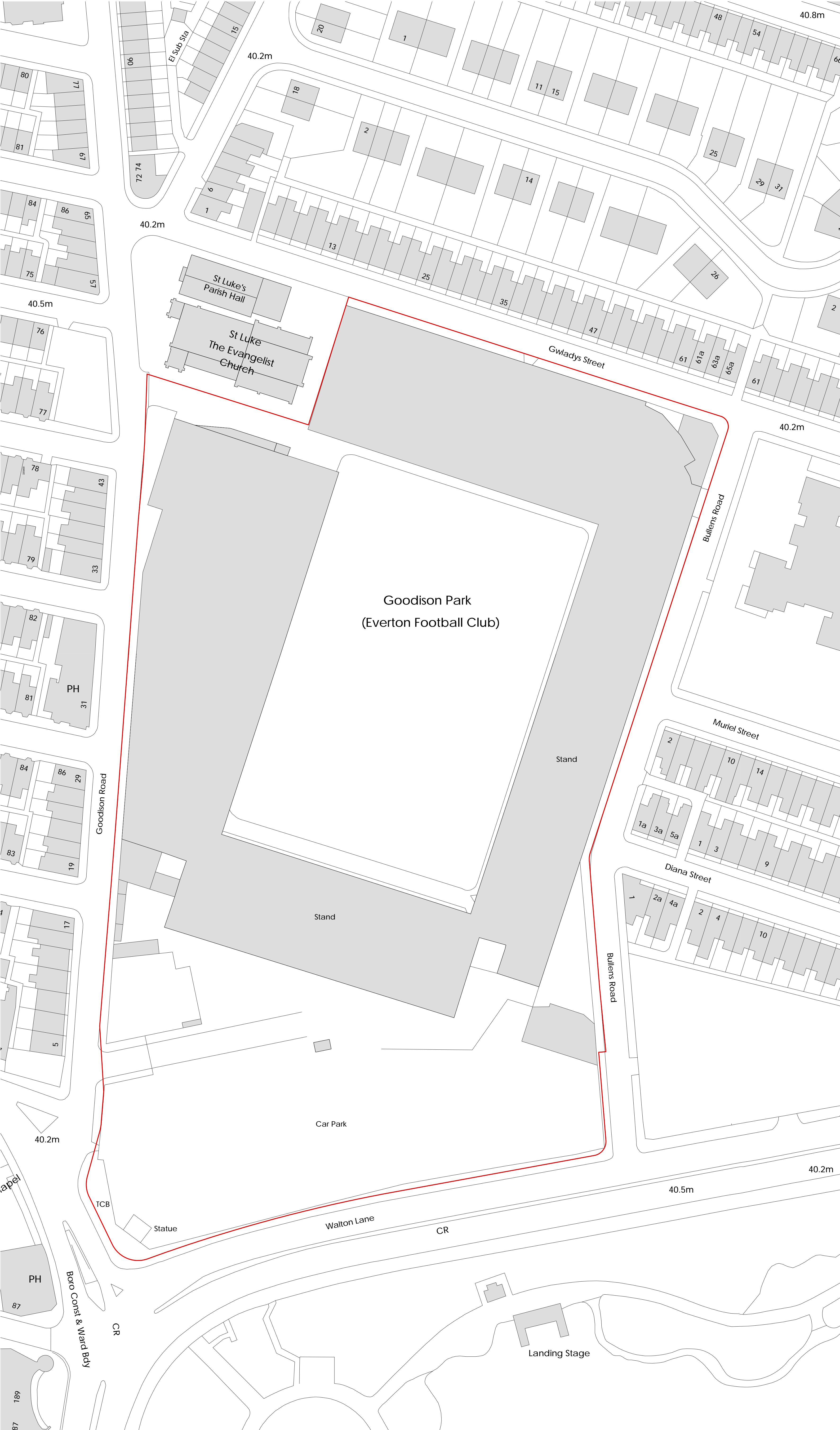
Existing Site Plan Scale 1:500
