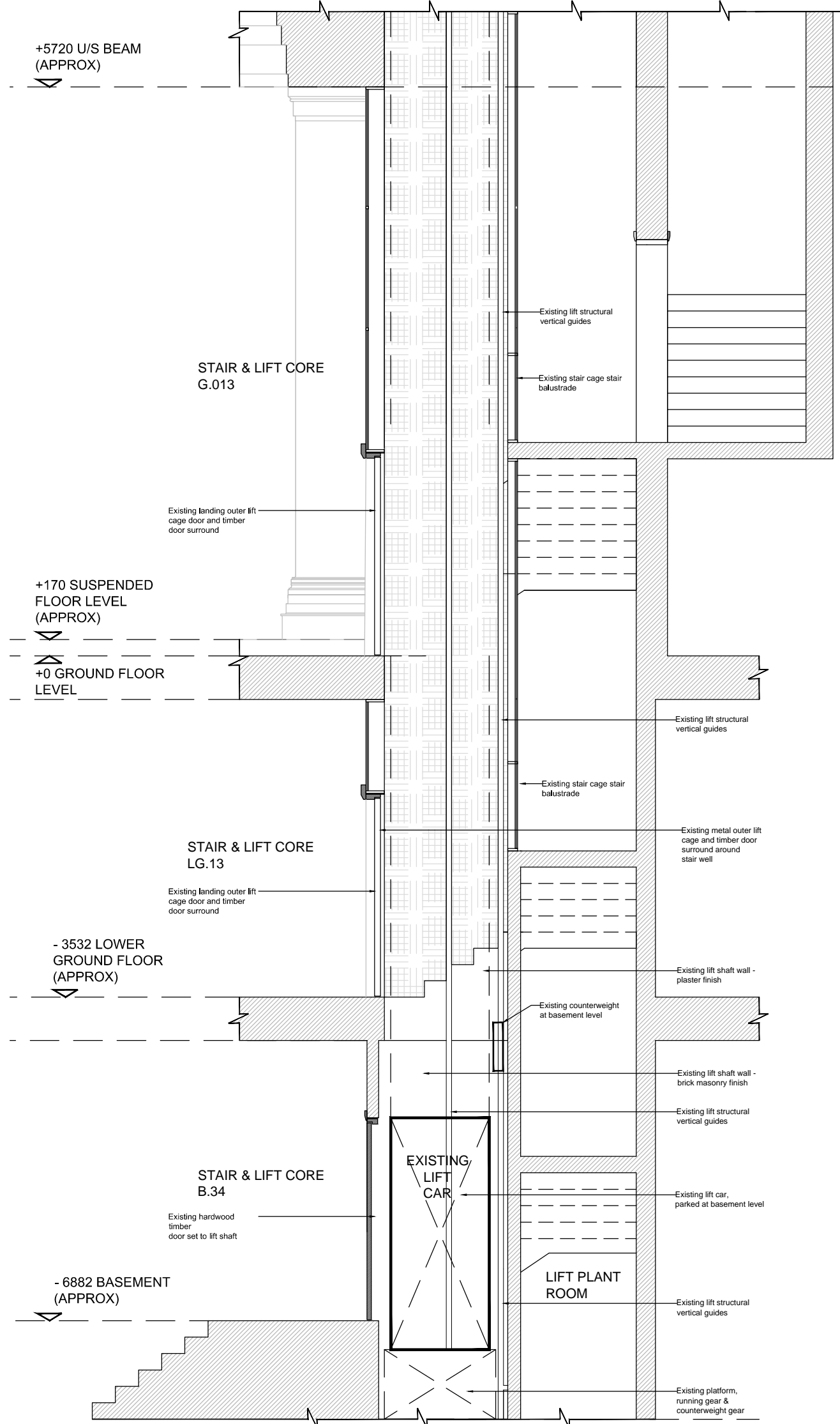
EXISTING LIFT SECTION A SCALE 1:50
