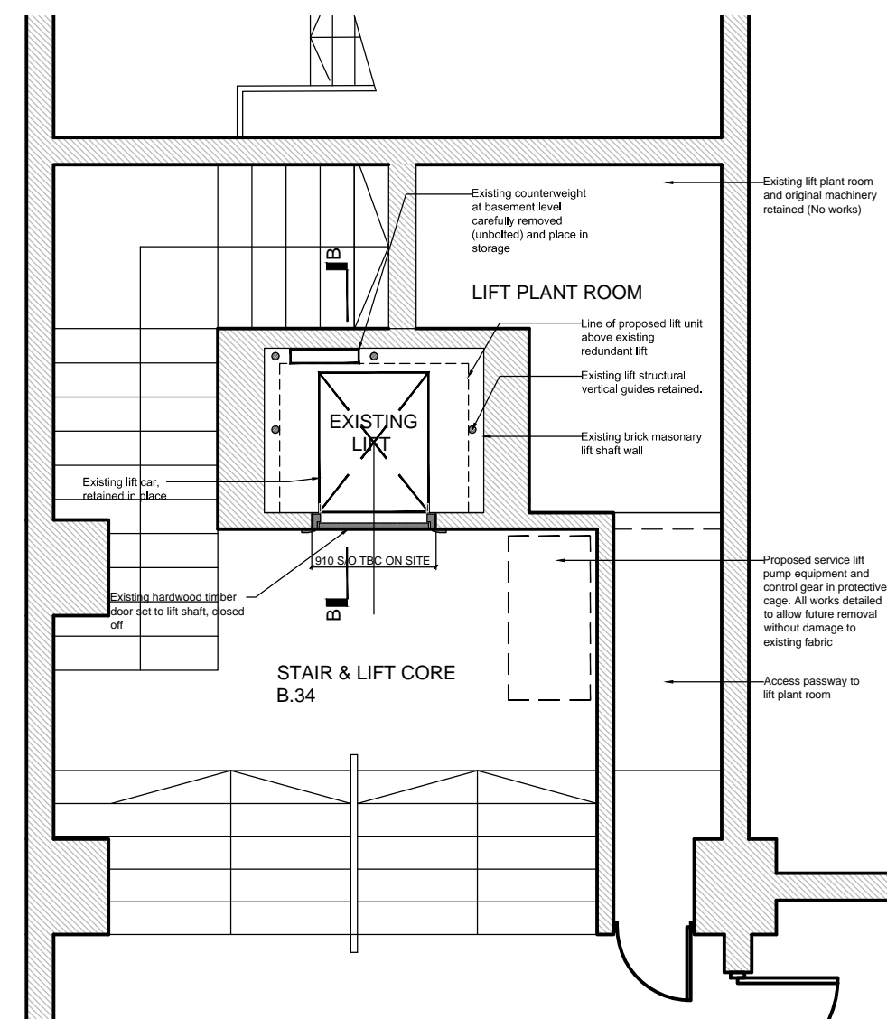
PROPOSED LOWER GROUND FLOOR LEVEL SCALE 1:50
