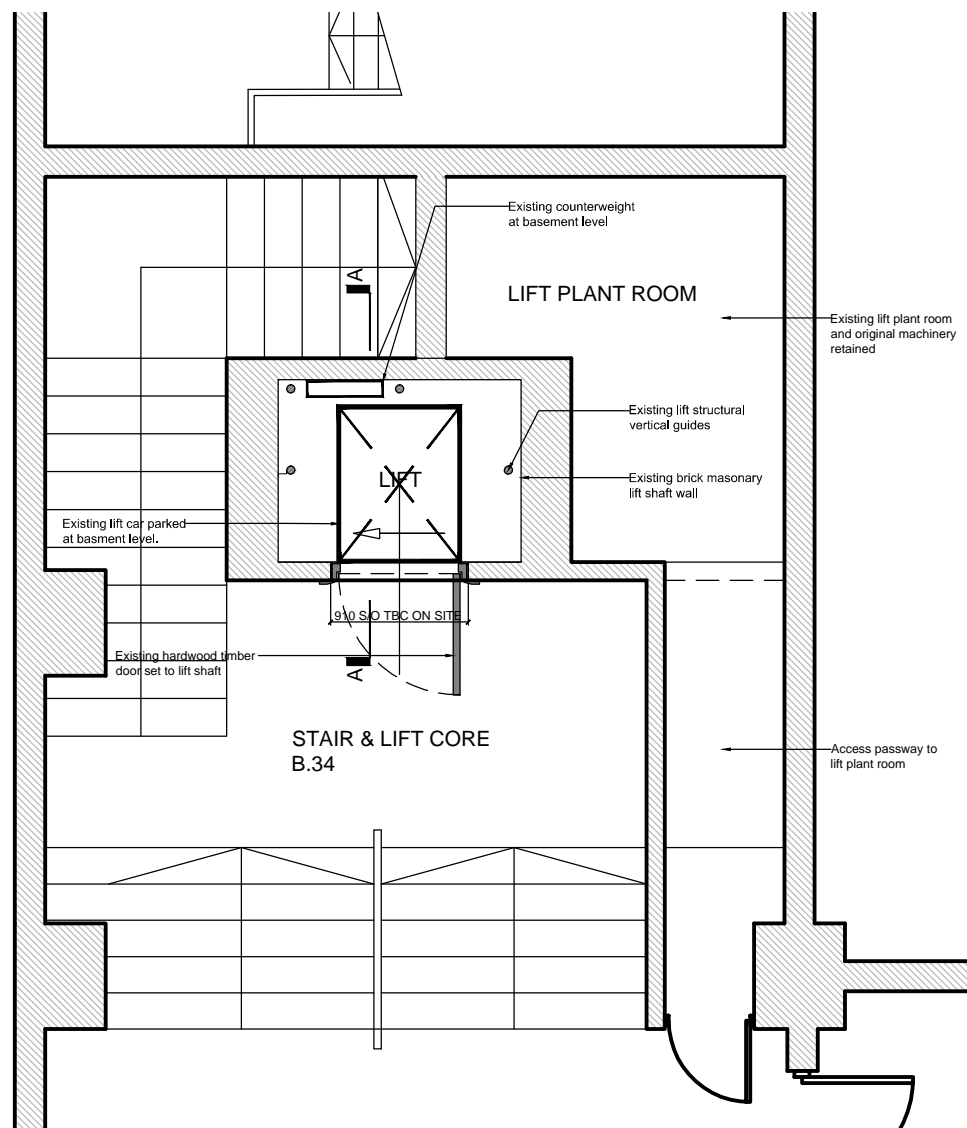
EXISTING LOWER GROUND FLOOR LEVEL SCALE 1:50
