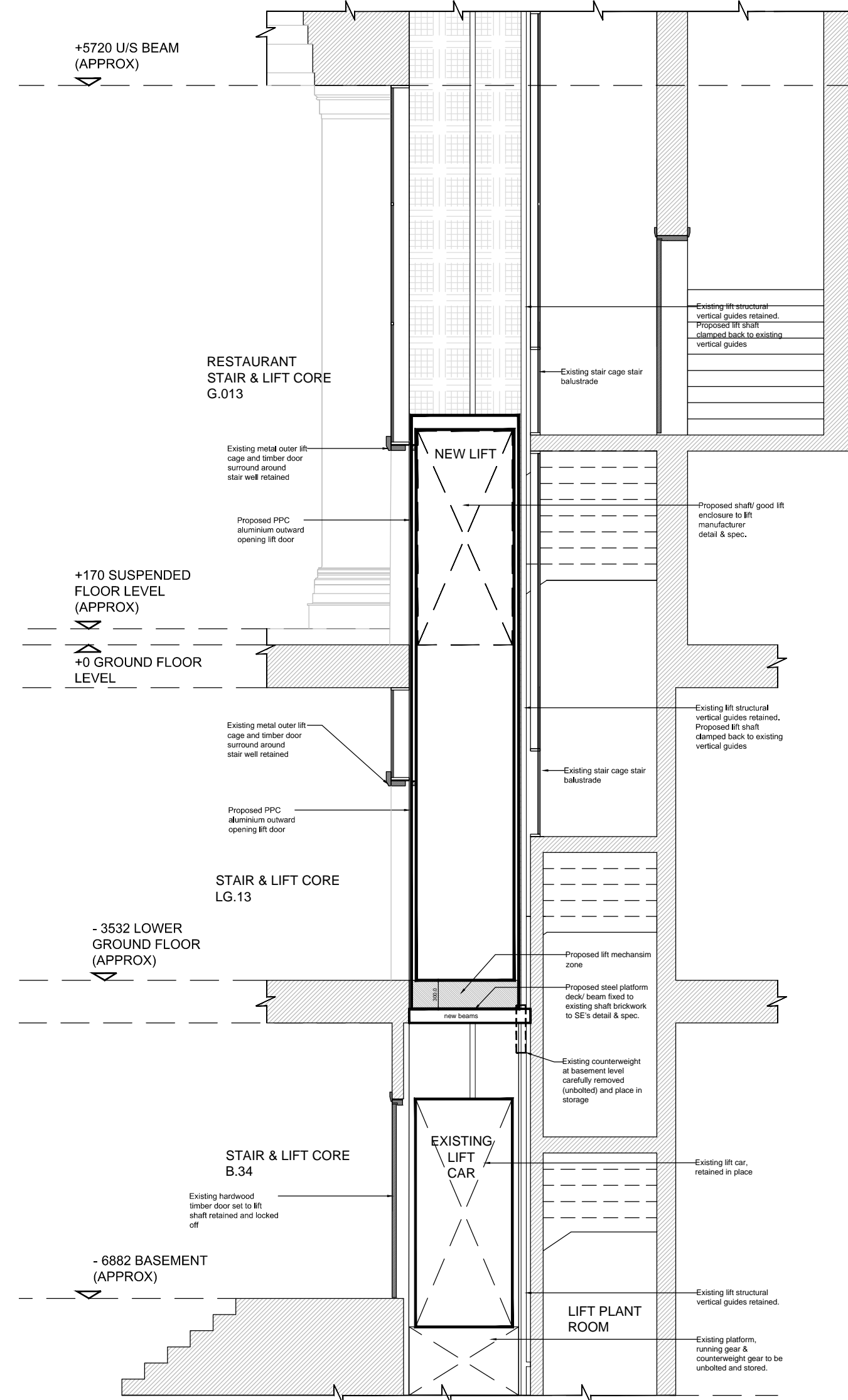
PROPOSED LIFT SECTION B SCALE 1:50
