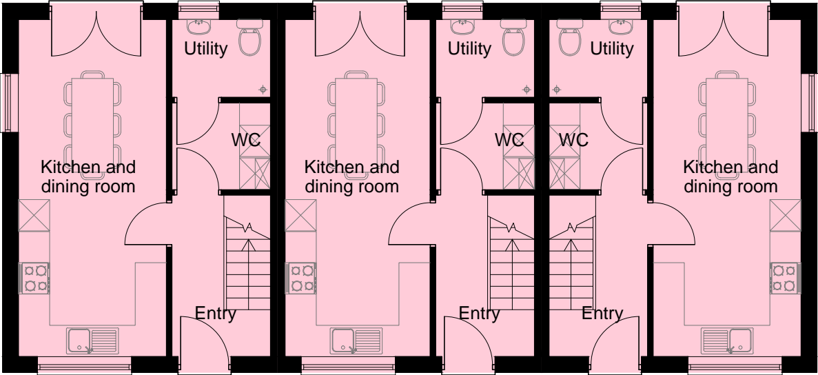
94.0m²/1,012ft² Ground floor
