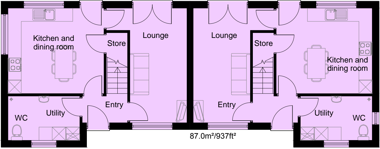
87.0m²/937ft² Ground floor
