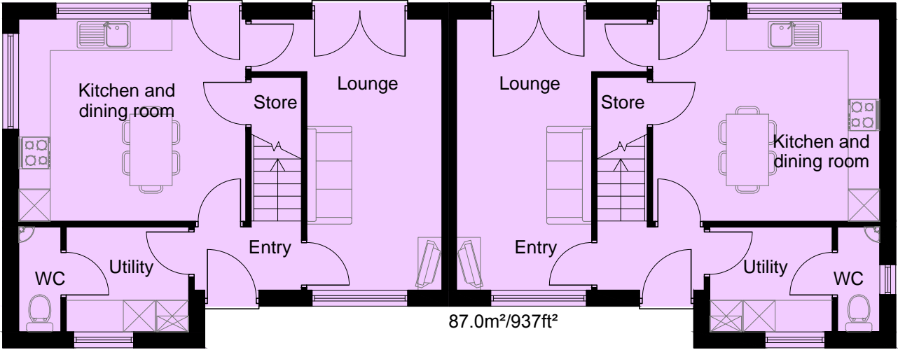
87.0m²/937ft² Ground floor
