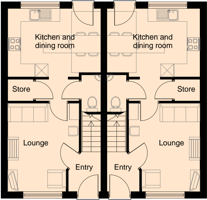
71.9m²/774ft² Ground floor
