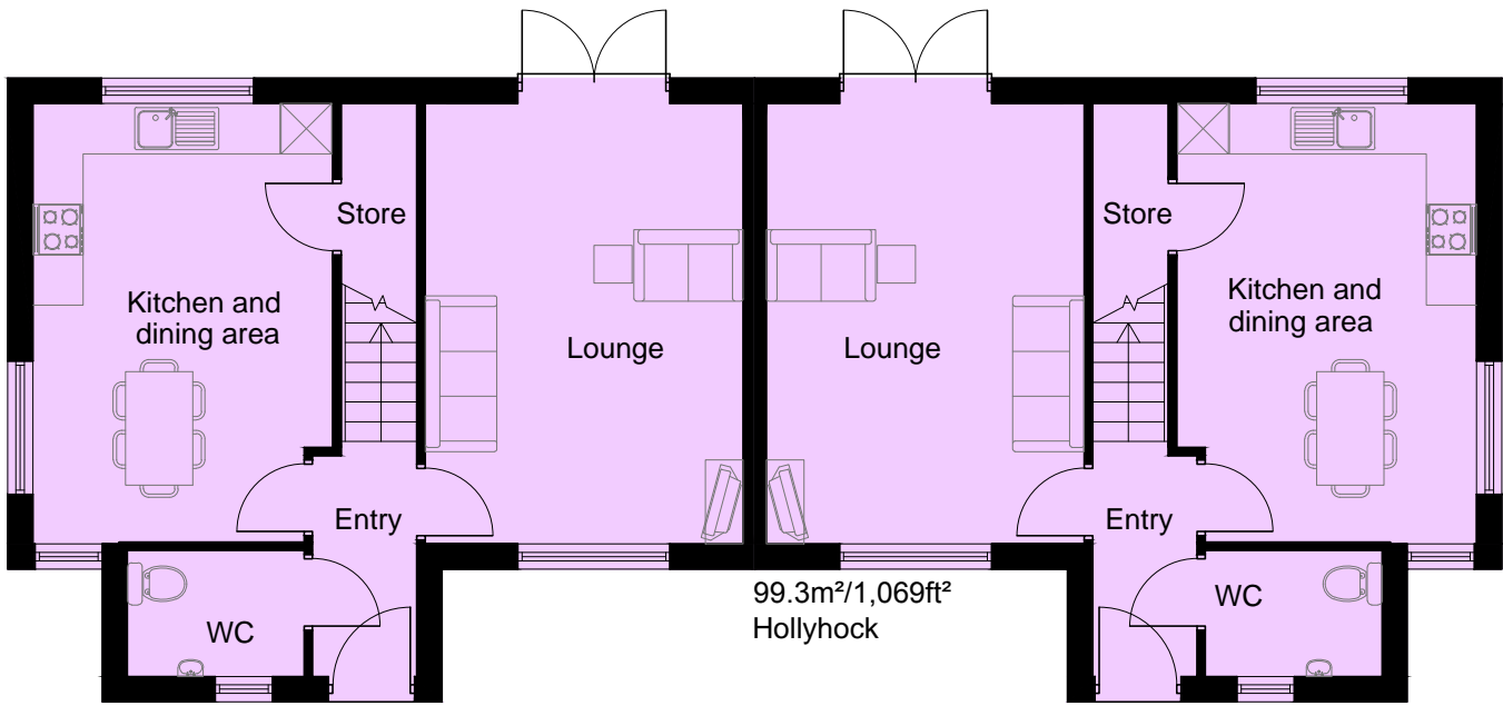
99.3m²/1,069ft² Hollyhock Ground floor
