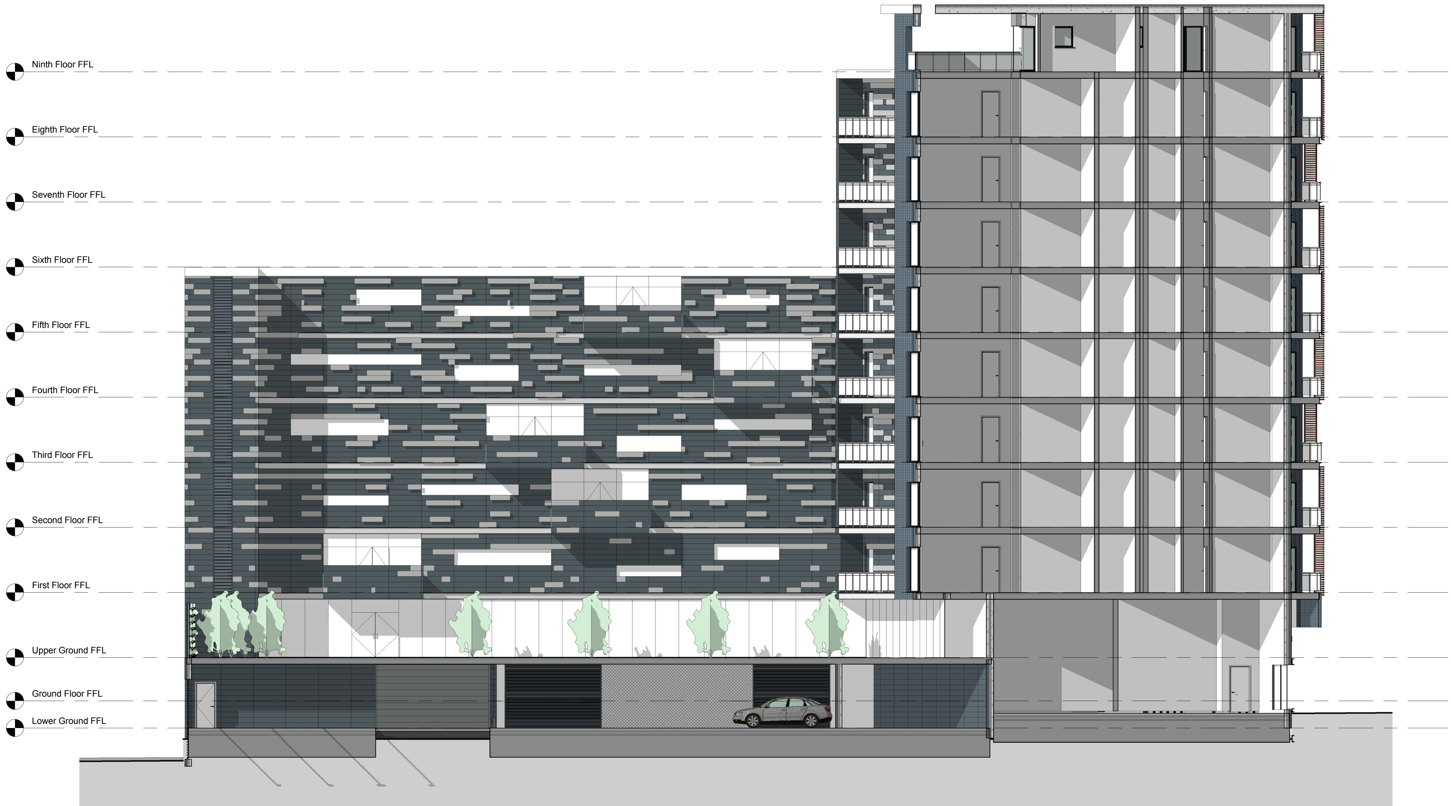
1 Proposed Section C-C 1 : 100
