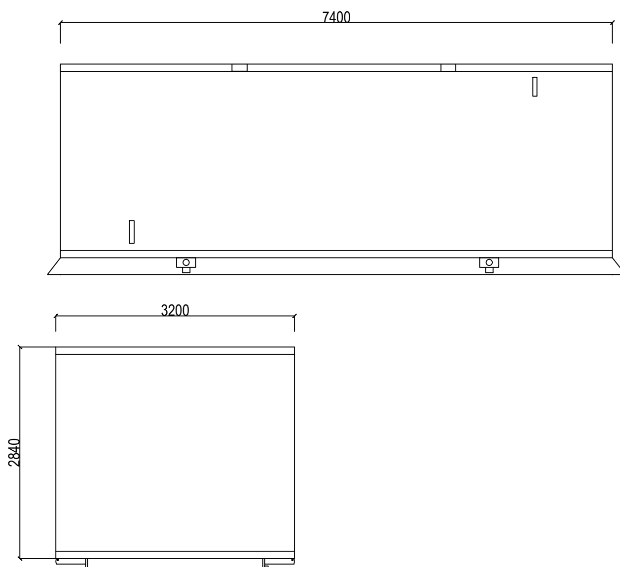
ELEVATIONS OF REB NOTE: FENCING IS OMITTED ON ELEVATIONS FOR CLARITY
