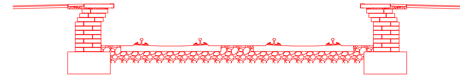
PLATFORM RISER WALL SECTION AA 1:50 NEW PLATFORM RISER WALLS ARE TO BE CONSTRUCTED OF CONCRETE BLOCK
