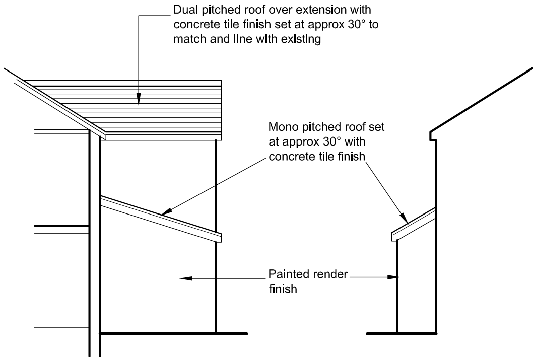
Proposed Side Elevations 1:100
