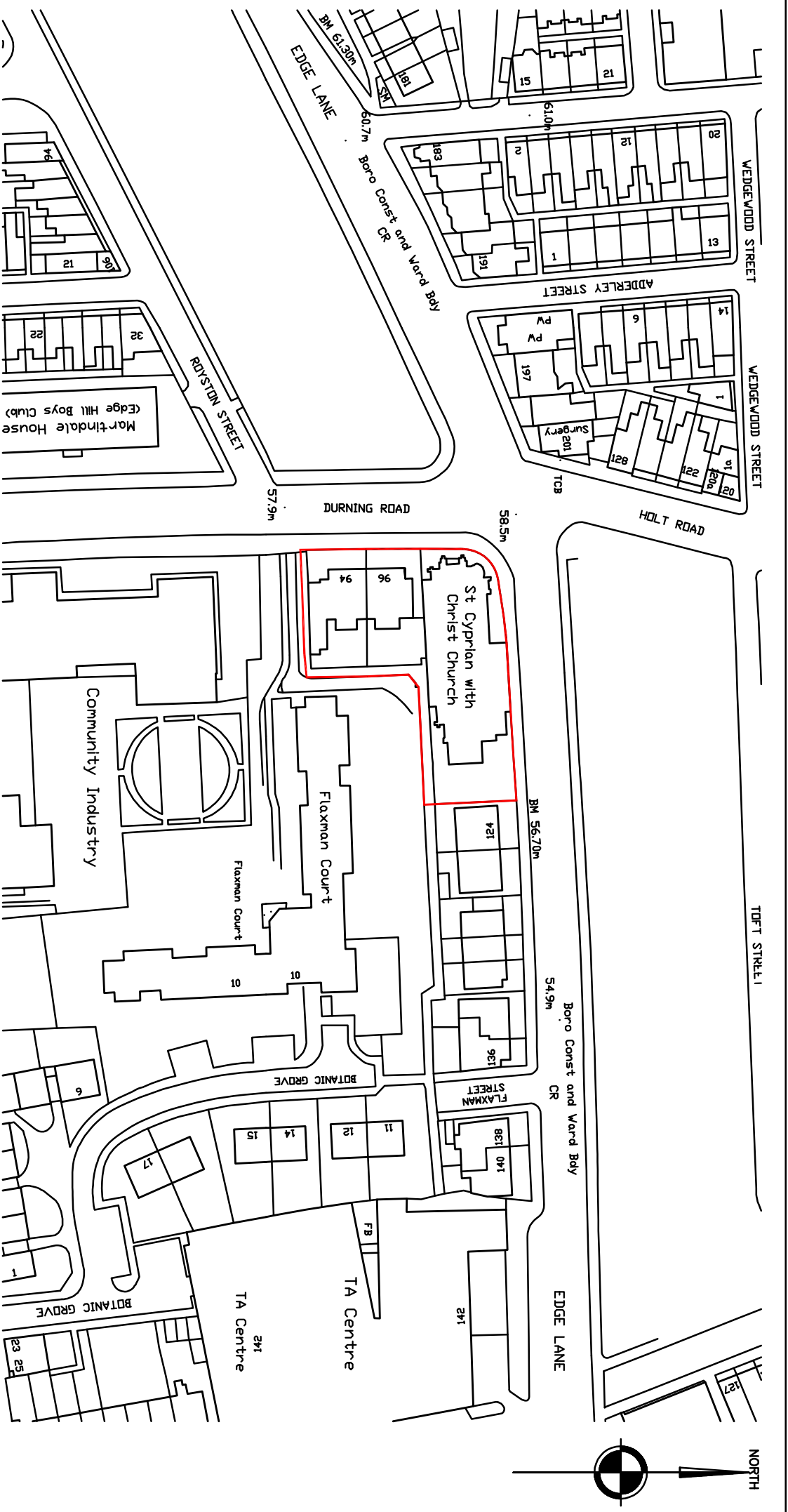
Location Plan Scale 1:1250
