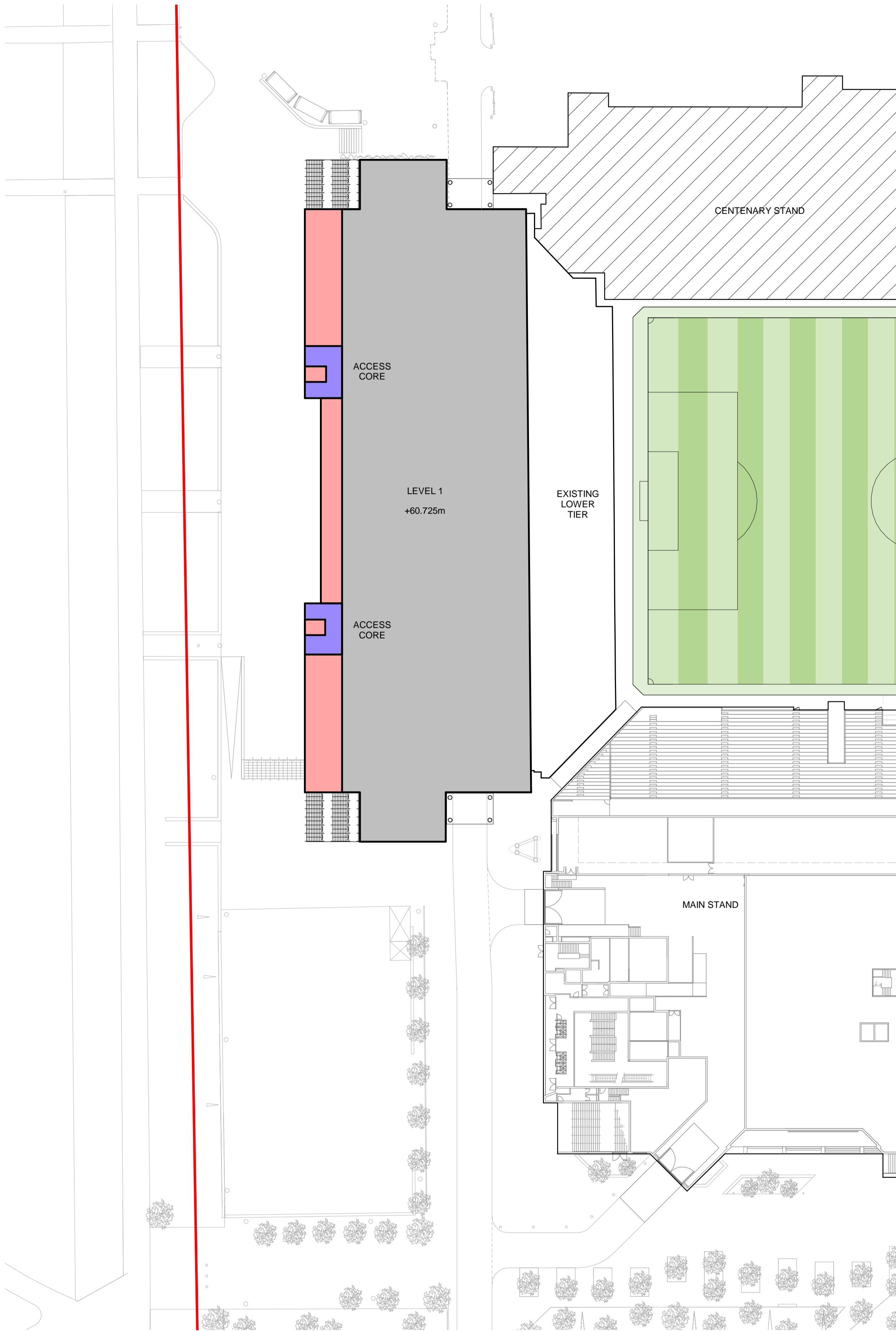
2 LEVEL 1 PLAN ANFIELD ROAD STAND PHASE 2
