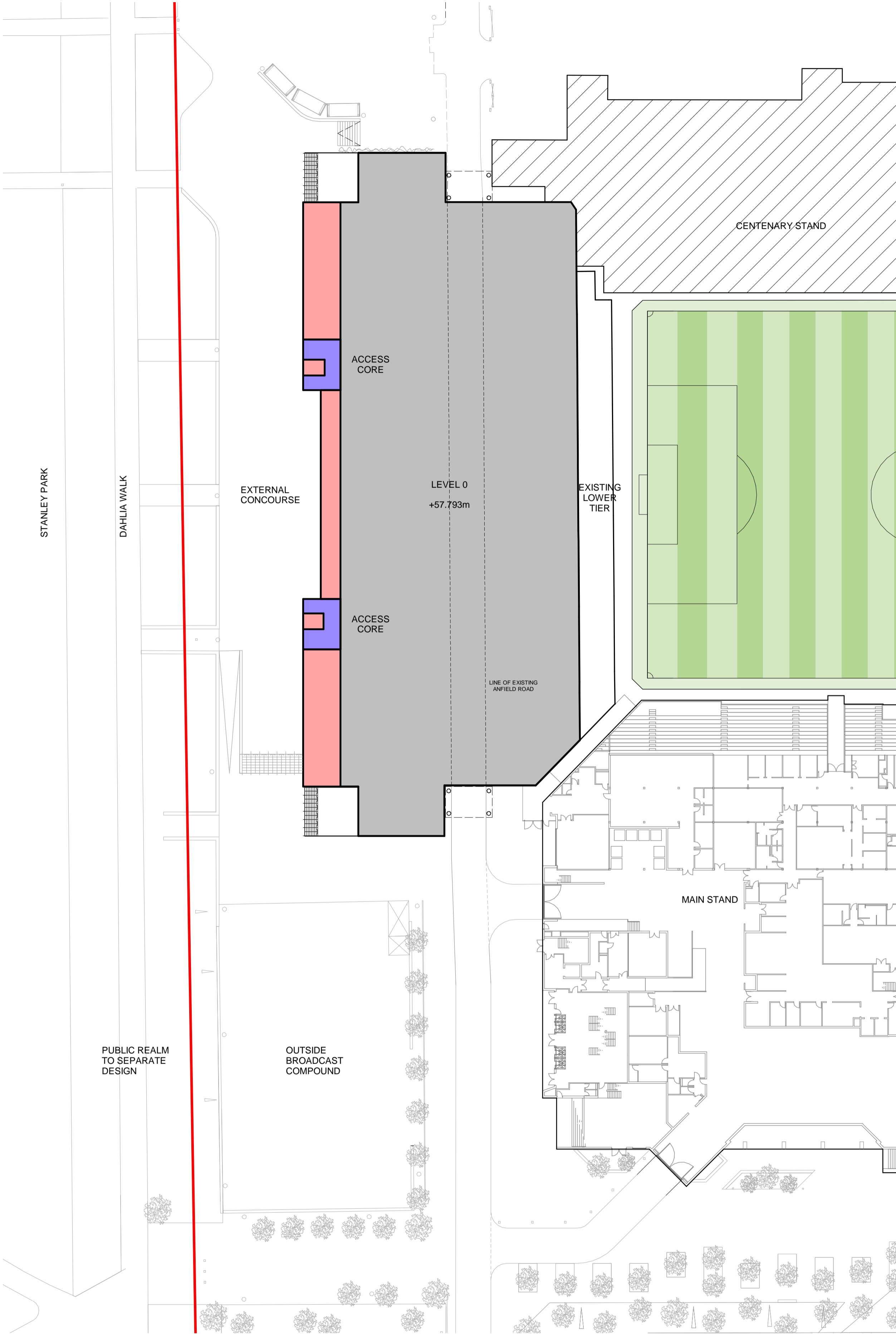
1 LEVEL 0 PLAN ANFIELD ROAD STAND PHASE 2
