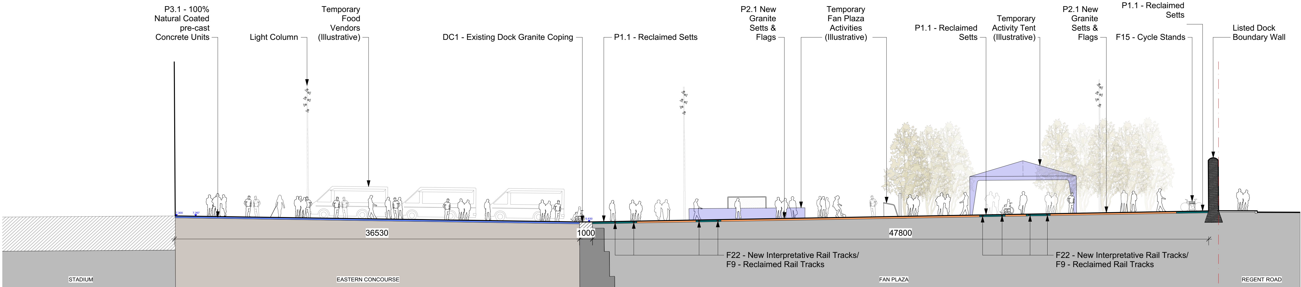
1 Section - Eastern (City) Concourse & Fan Plaza (Match Day Scenario) Scale 1:150 @ A0
