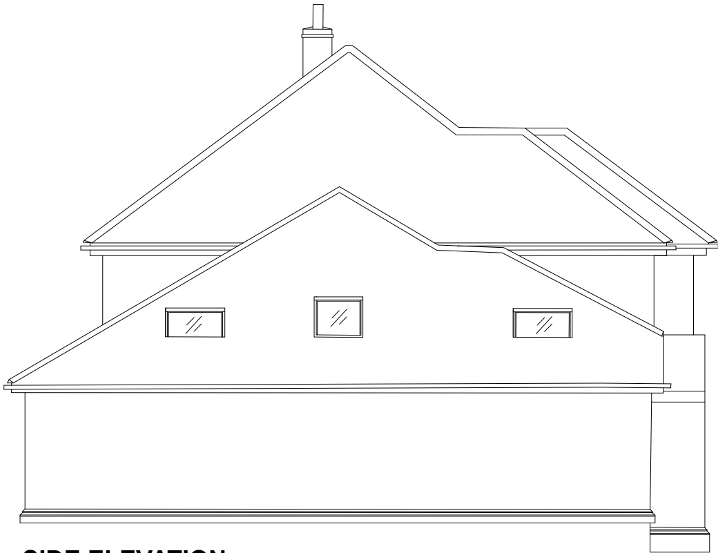
SIDE ELEVATION
