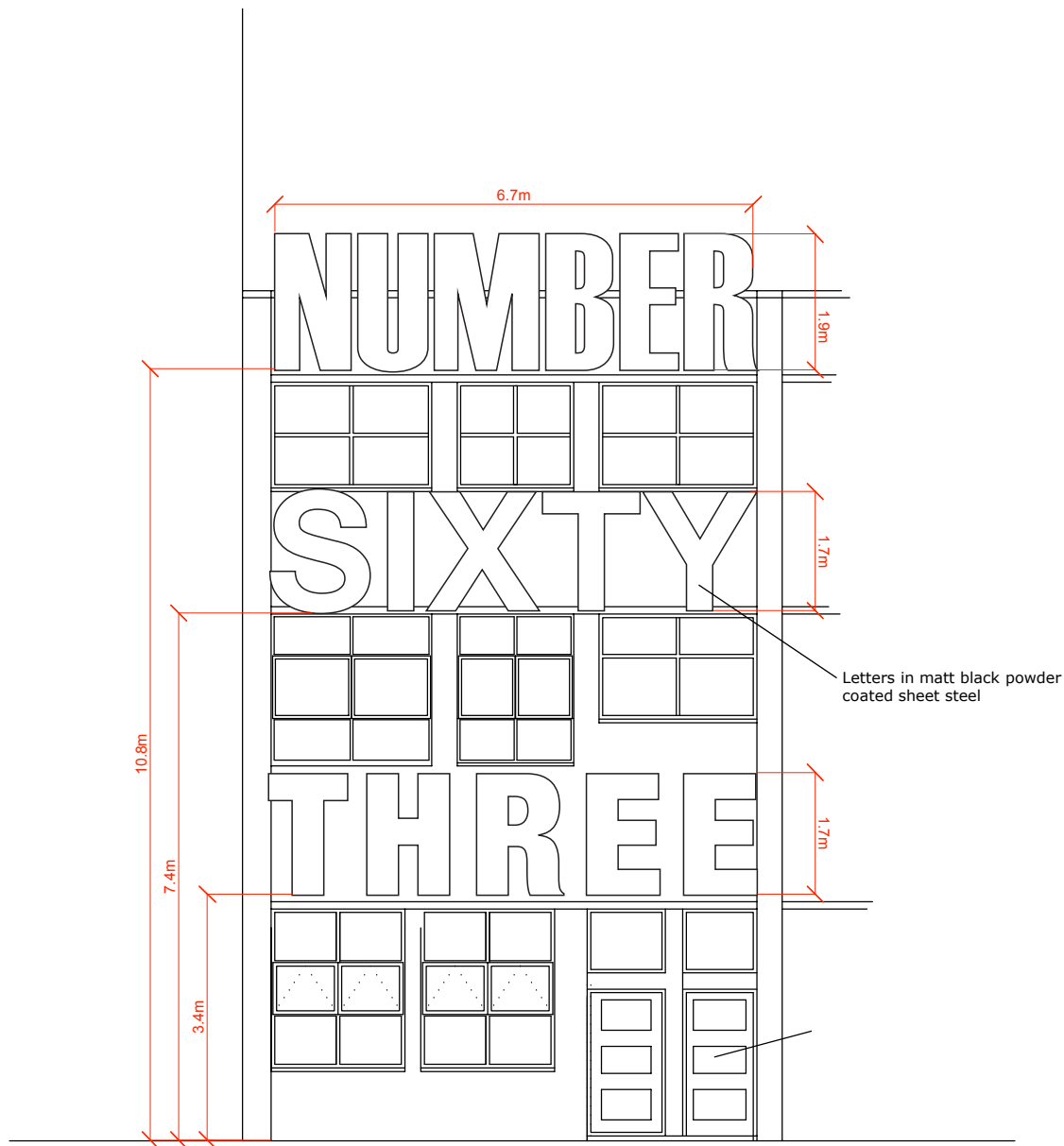
FRONT ELEVATION
