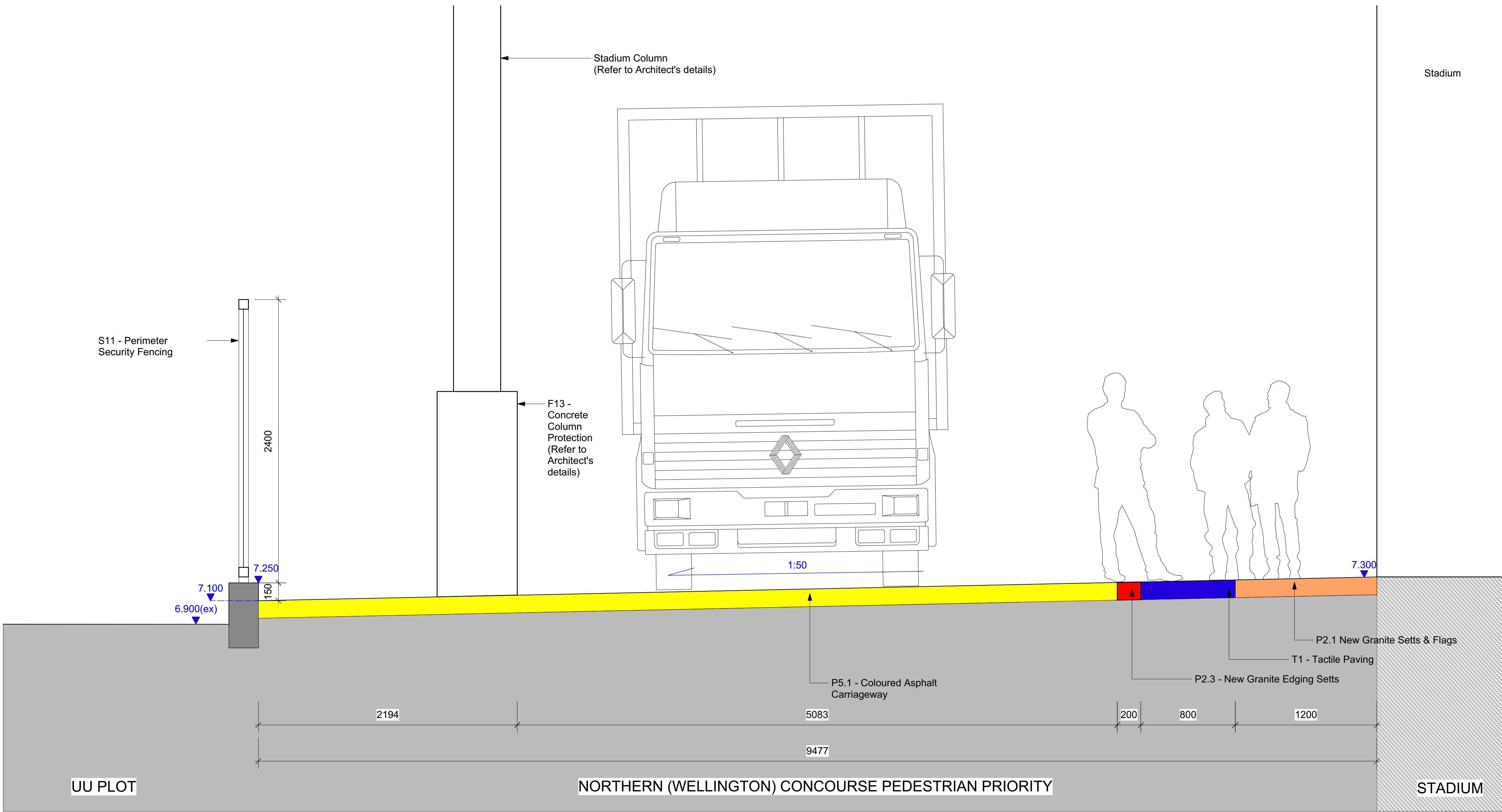
1 Section - Northern (Wellington) Concourse Scale 1:20 @ A0
