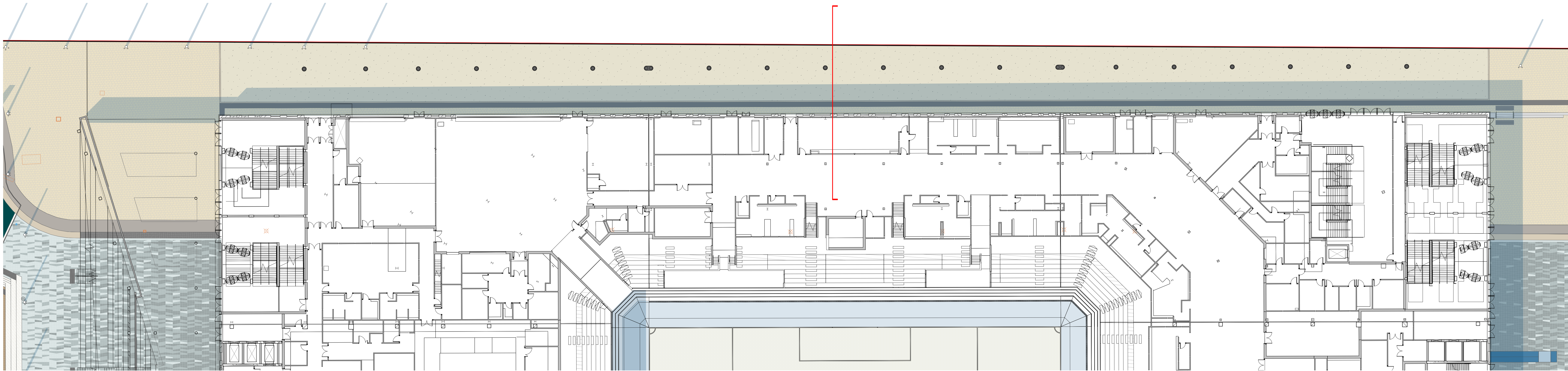
2 Plan - Northern (Wellington) Concourse Scale 1:250 @ A0
