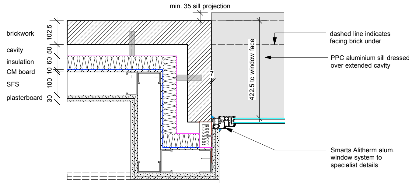
DETAIL D - deep reveal window jamb to SFS [ground level]
