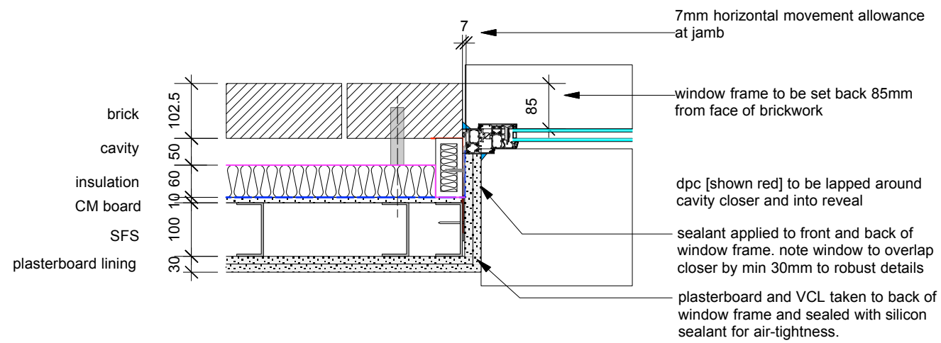
DETAIL A - standard window jamb to SFS [ground level]
