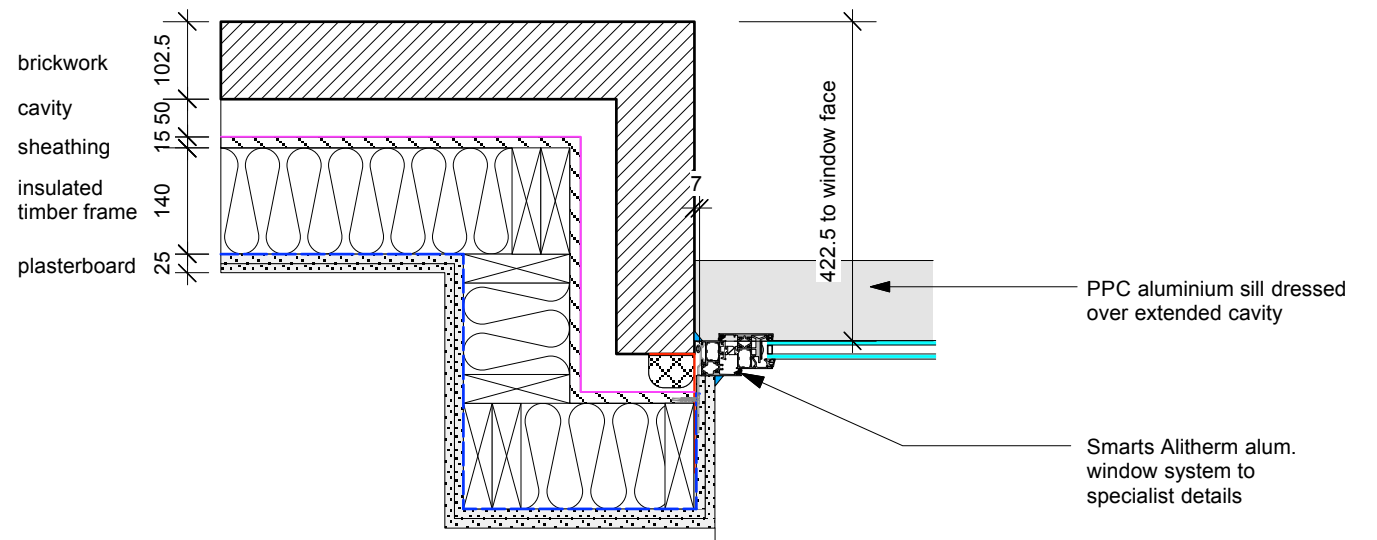
DETAIL E - deep reveal window jamb to timber frame [upper levels]
