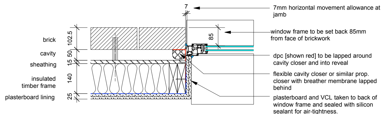
DETAIL C - standard window jamb to timber frames [upper levels]
