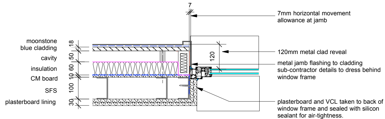
DETAIL B - metal cladding window jamb
