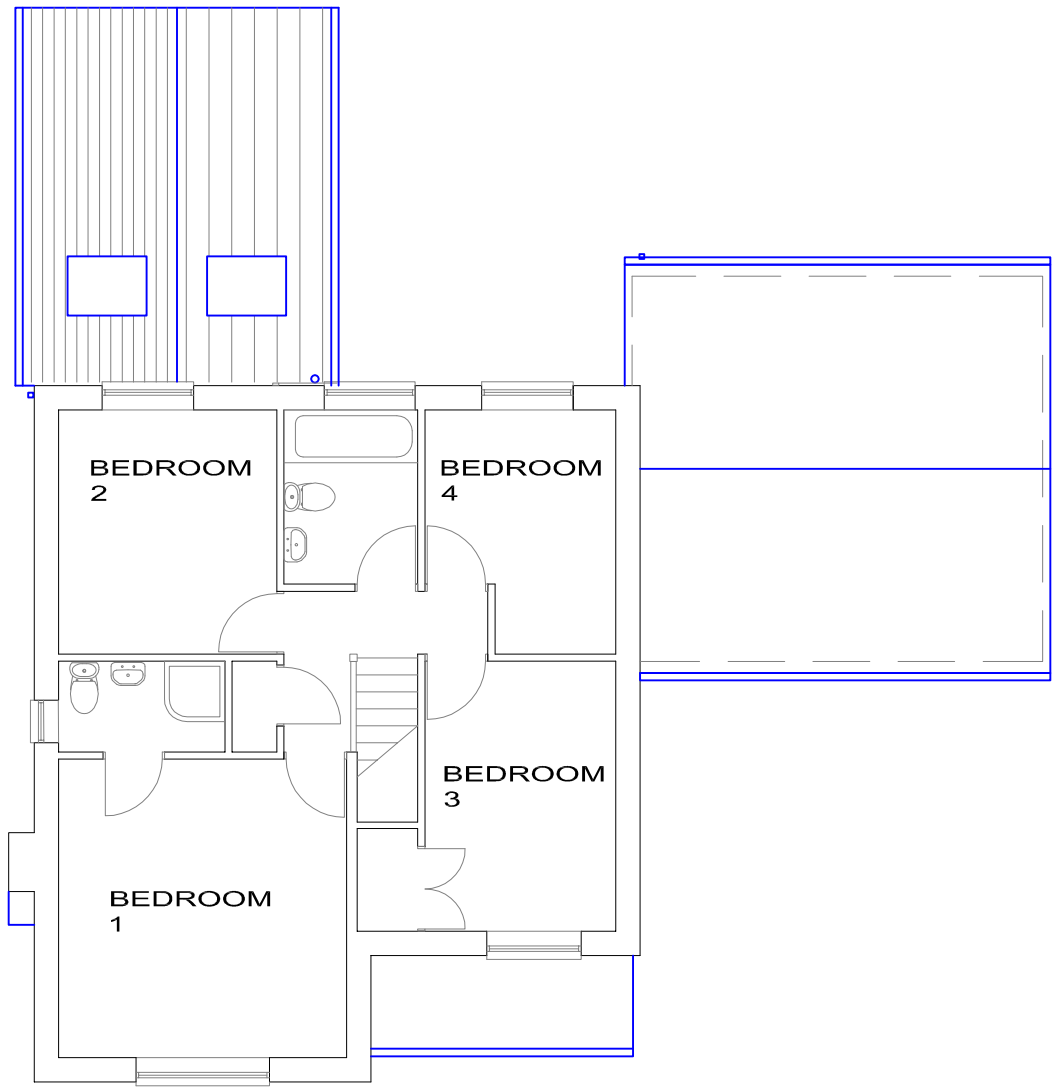
FIRST FLOOR 1:100
