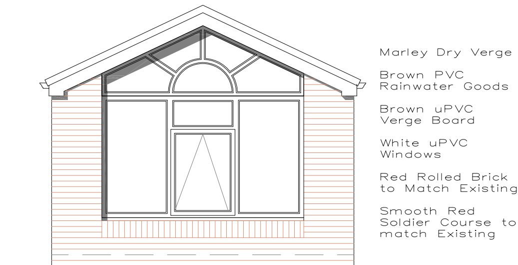
REAR ELEVATION 1:50
